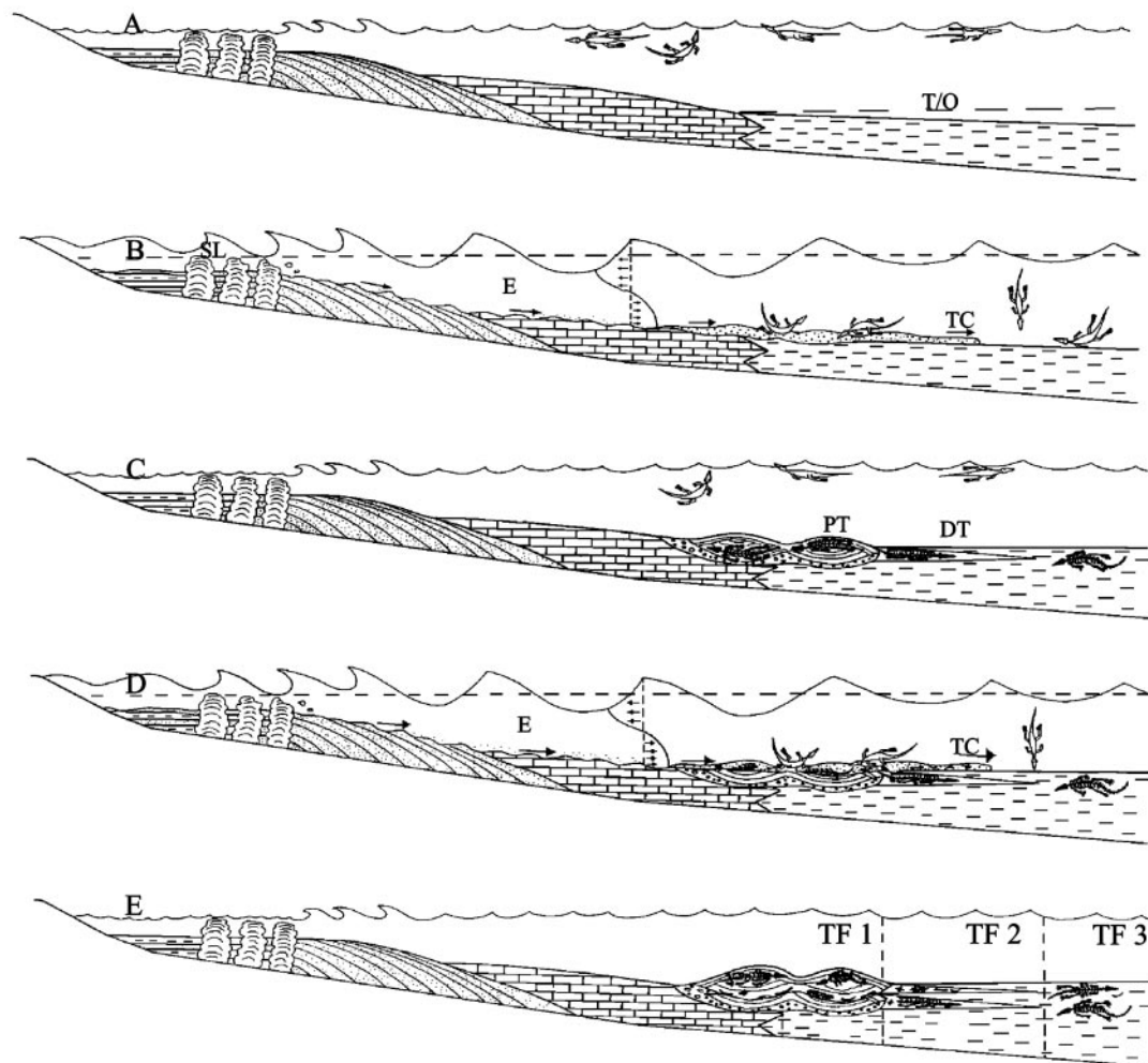
FIGURE 6 Cartoon showing idealised onshore-offshore sections in the Whitehill-Irati Sea, showing the relation between the different facies and the processes influencing on the formation of mesosaur taphocenosis. Note the development of carbonate facies in the marginal littoral zones (including stromatolites and bioclastic sands) in opposition to the predominance of fine grained silicilastic deposits in the offshore areas. A to E display a sequence of taphofacies' generation along time. A) Normal conditions with mesosaurs living at the surface waters and water stratification because of the development of a thermo-oxicleine (T/O). B) Major storm event affecting the sea (SL) and producing a combined flow (waves and currents); thermo-oxicleine break and upwelling of anoxic waters; erosion of previously deposited sediments (E), reworking and suspension of biogenic and sedimentary material; transport to offshore zones by turbiditic currents (TC); mesosaurs dying, reaching the bottom and being buried. C) Normal conditions; proximal (PT) and distal (DT) tempestite deposition at shallow parts of the basin; little bottom disturbance at deeper basin zones. D) New major storm event reworking the previous deposits and associated buried biogenic material that had resulted from B and C; new mesosaurs' carcasses reaching the bottom and being buried. E) Normal conditions: formation of new tempestites overlying the older ones (produced in C). Taphofacies 1 (TF1) - proximal tempestite zone; Taphofacies 2 (TF2) - distal tempestite zone; Taphofacies 3 (TF3) - no tempestite generation.
